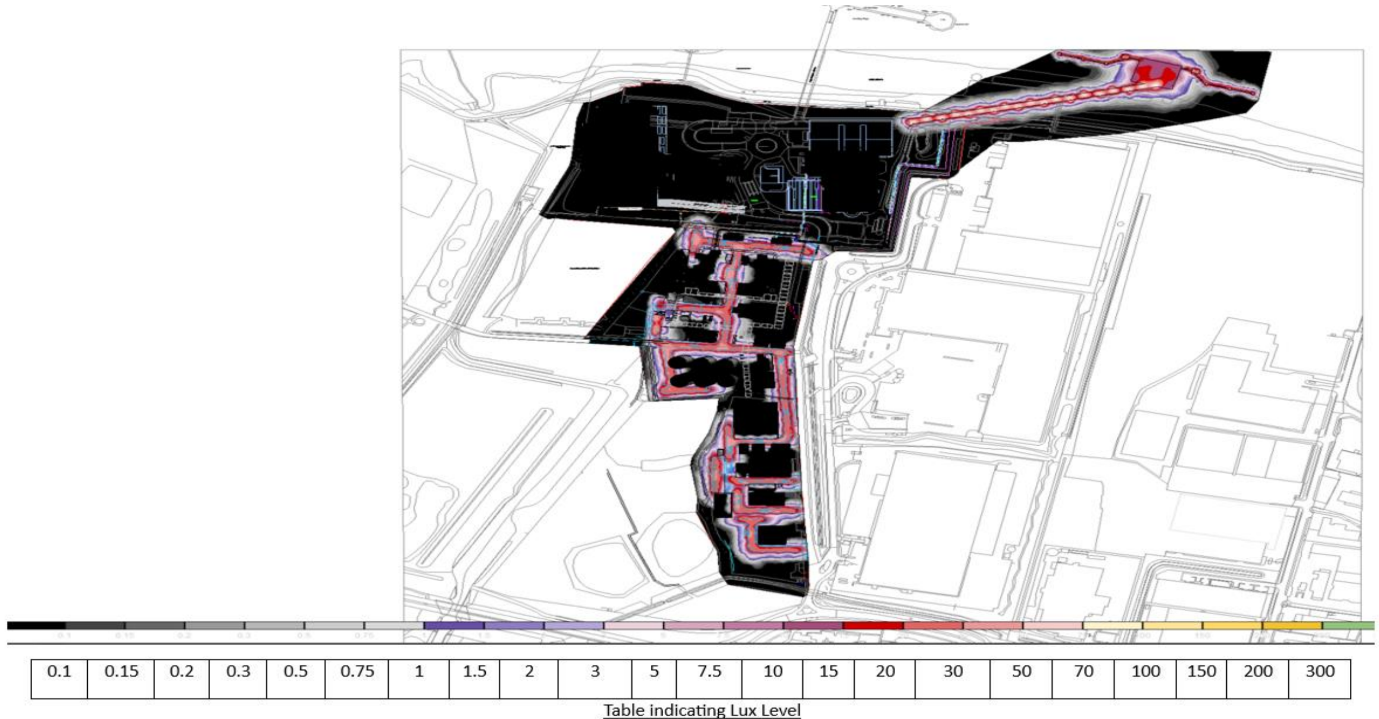
Figure 4-1 – Indicative Site Layout Calculated Lux Levels
